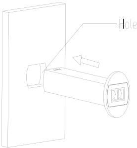
Recess Mount
