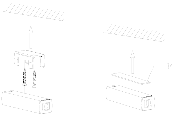
Surface Mount
