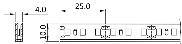
12Vdc strip cutting length
