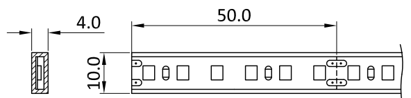
24Vdc strip cutting length
