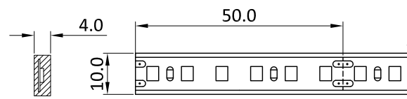
24Vdc strip cutting length
