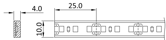
12Vdc strip cutting length
