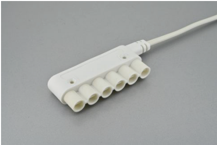
D8W V6 6way Splitter max 10A 250V AC max 5A per connector
